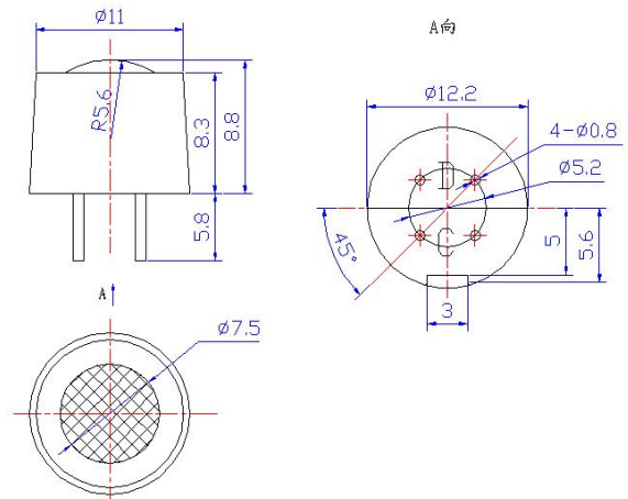
Fig1. Sensor Structure
