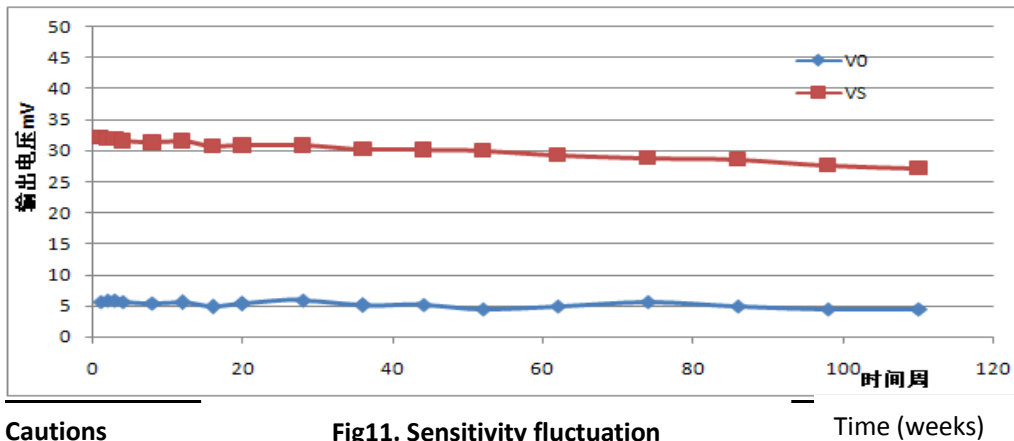
Fig11. Sensitivity fluctuation
