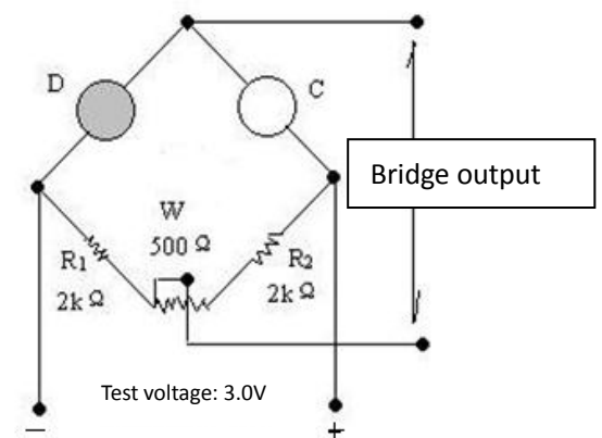
Fig2. Basic Test Circuit
