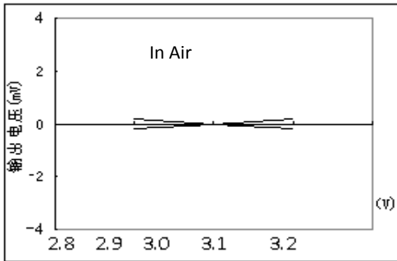
Fig9.Zero point with different voltage
